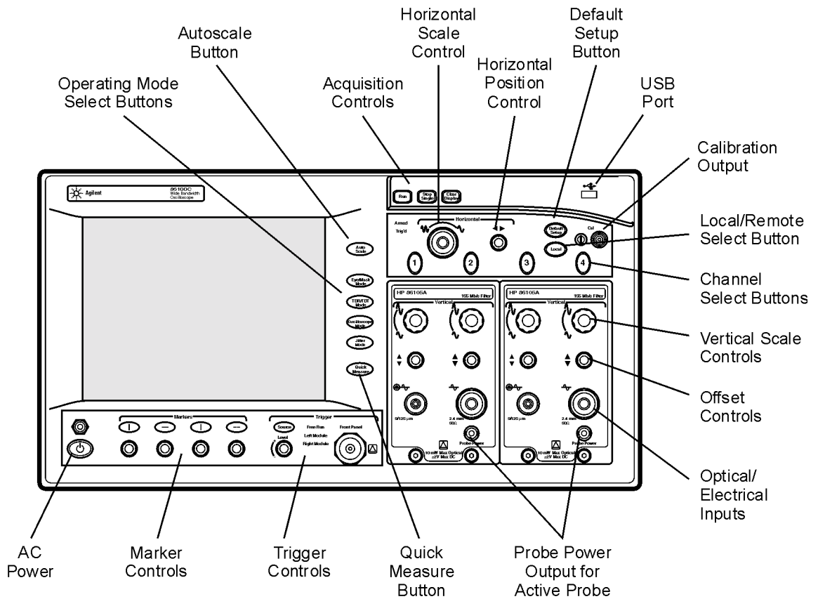
Figure 2-4. Front-Panel Features
