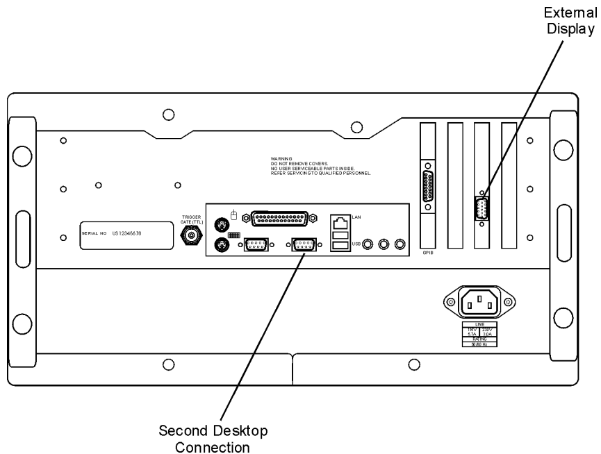
Figure 1-23. External Monitor Connector
